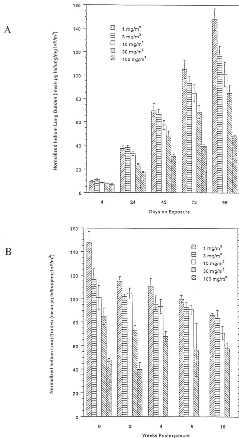
Figure 2 Normalized Lung Burden of Indium in Rats During 14 Weeks of Exposure (A) or During the 16 Weeks Following Exposure (B) to Indium Phosphide. Data are presented as mean \pm standard deviation.
