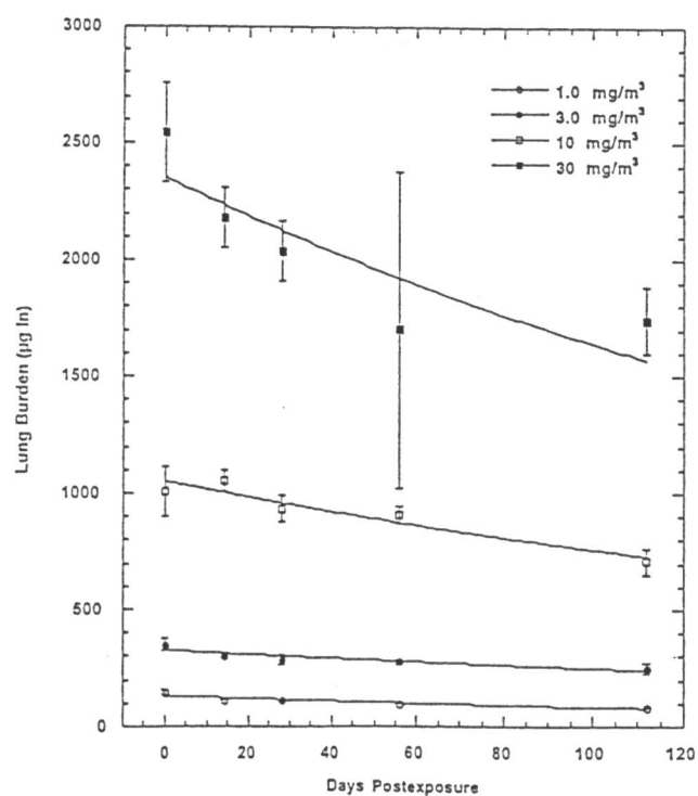
Figure 1 Lung Burden of Indium in Rats During 14 Weeks Exposure (A) or During the 16 Weeks Following Exposure (B) to Indium Phosphide. Data are presented as mean \pm standard deviation. Curves represent the fit of the lung deposition and clearance model to the data.
