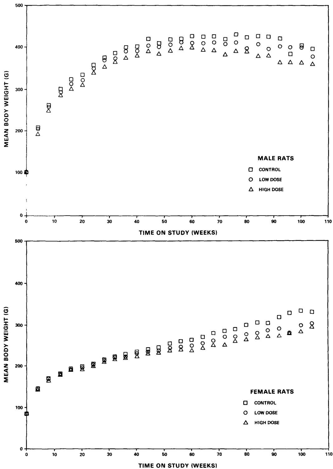
Figure 1. Growth Curves for Rats Fed Diets Containing Caprolactam
